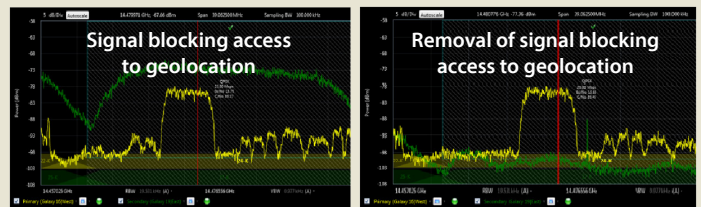
▲ Display shows signal blocking access to geolocation and then being removed using Monics satID.
