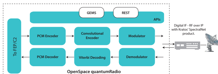
OpenSpace quantumRadio System Architecture
