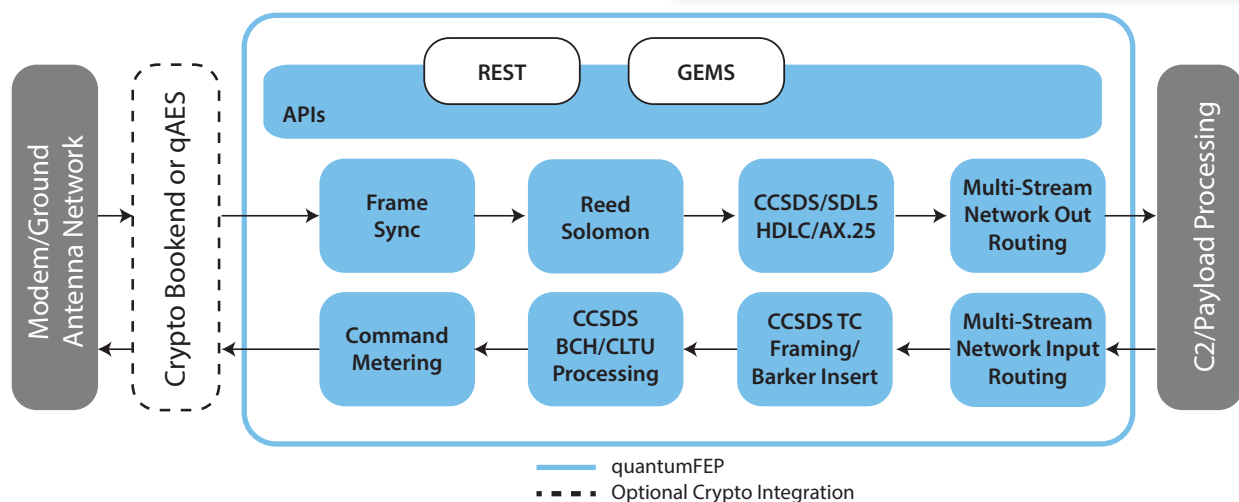
OpenSpace quantumFEP high-level architecture.
