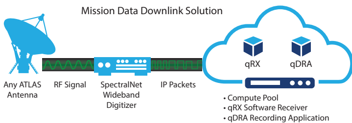
ATLAS' system architecture for wideband satellite signal processing in software for mission data downlink.
