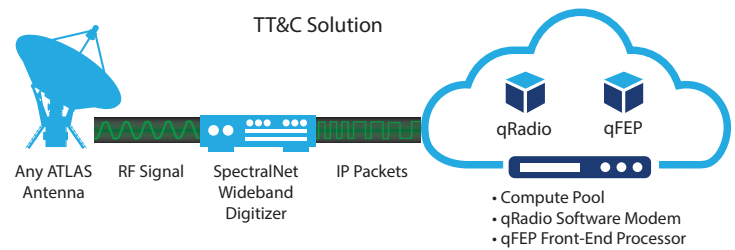
ATLAS' system architecture for narrowband satellite signal processing in software for TT&C and narrowband payloads.
