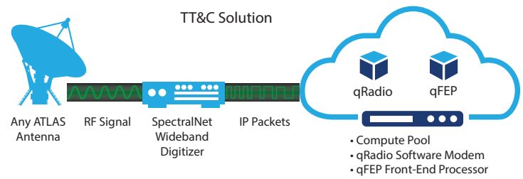
ATLAS' system architecture for narrowband satellite signal processing in software for TT&C and narrowband payloads.
